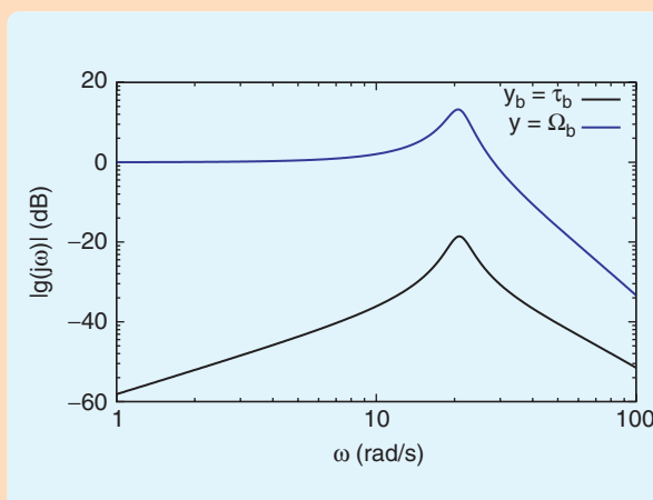
FIGURE S2 Frequency response for the Quanser experiment. The numerical values of Table S1 combined with the bond graph of Figure S1 yield the frequency response of y = \Omega_b and y_b = \tau_b , measured in rad/s and N-m, respectively, to the equivalent system input u_0 , measured in rad/s; the resonant peak corresponds to the flexure natural frequency of about 20 rad/s.
