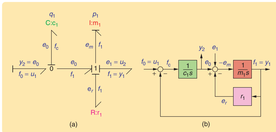
FIGURE 7 System causality. (a) Causal bond graph with causality completed on each component. As indicated by the causal strokes, the C : c 1 component has its preferred causality of flow in and effort out, the I : m 1 component has its preferred causality of effort in and flow out, whereas the R : r 1 component has, in this system, a causality of effort out and flow in. Annotations such as q_1 are for clarity and are not part of the bond-graph notation. (b) Block-diagram. The input and output of each component corresponds to the causal stroke on the bond-graph components of (a); the C and I components are in integral causality since they lead to block-diagram integrators. From Table 1, the associated states are the integrated flow q_1 and integrated effort p_1 . The block diagram and bond graph share the same color coding to indicate the corresponding elements.
